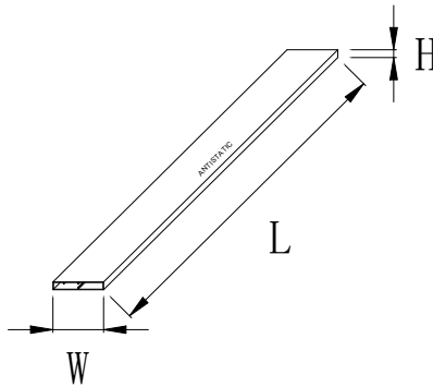
Fig.1- Tube pack for TO-247-4 full
